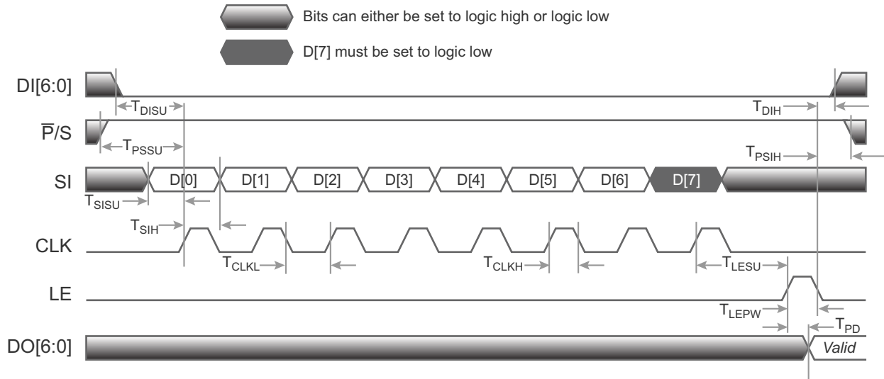
Figure 4 • Latched Parallel/Direct Parallel Timing Diagram
